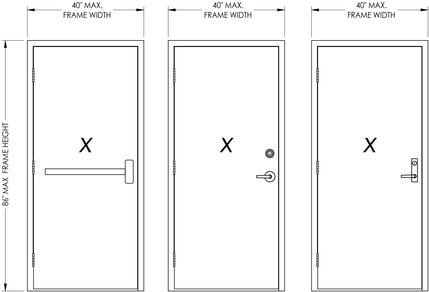
RIM PANIC BAR EXIT DEVICE w/ DEADBOLT
